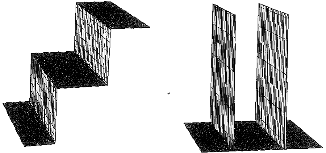
FIGURE 12.18: Behavior of the entire system for the simulation with an ordered initial configuration, Figure 12.16. Time goes from left to right, block number from front to back, and the vertical axis is position (left figure) or velocity (right figure). The time span here is t = 0 to 500, the same as that covered in Figure 12.16.
