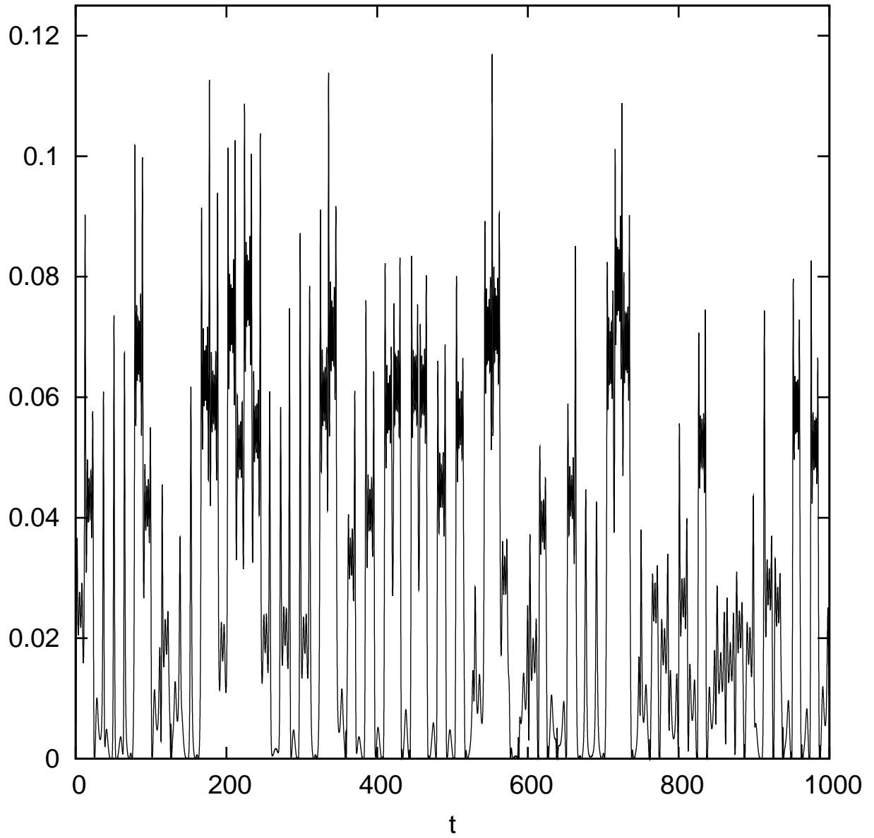
Orbiting Dumbbell Problem Elliptical Orbit Rotational Kinetic Energy -- Tolerance=10(-12)
