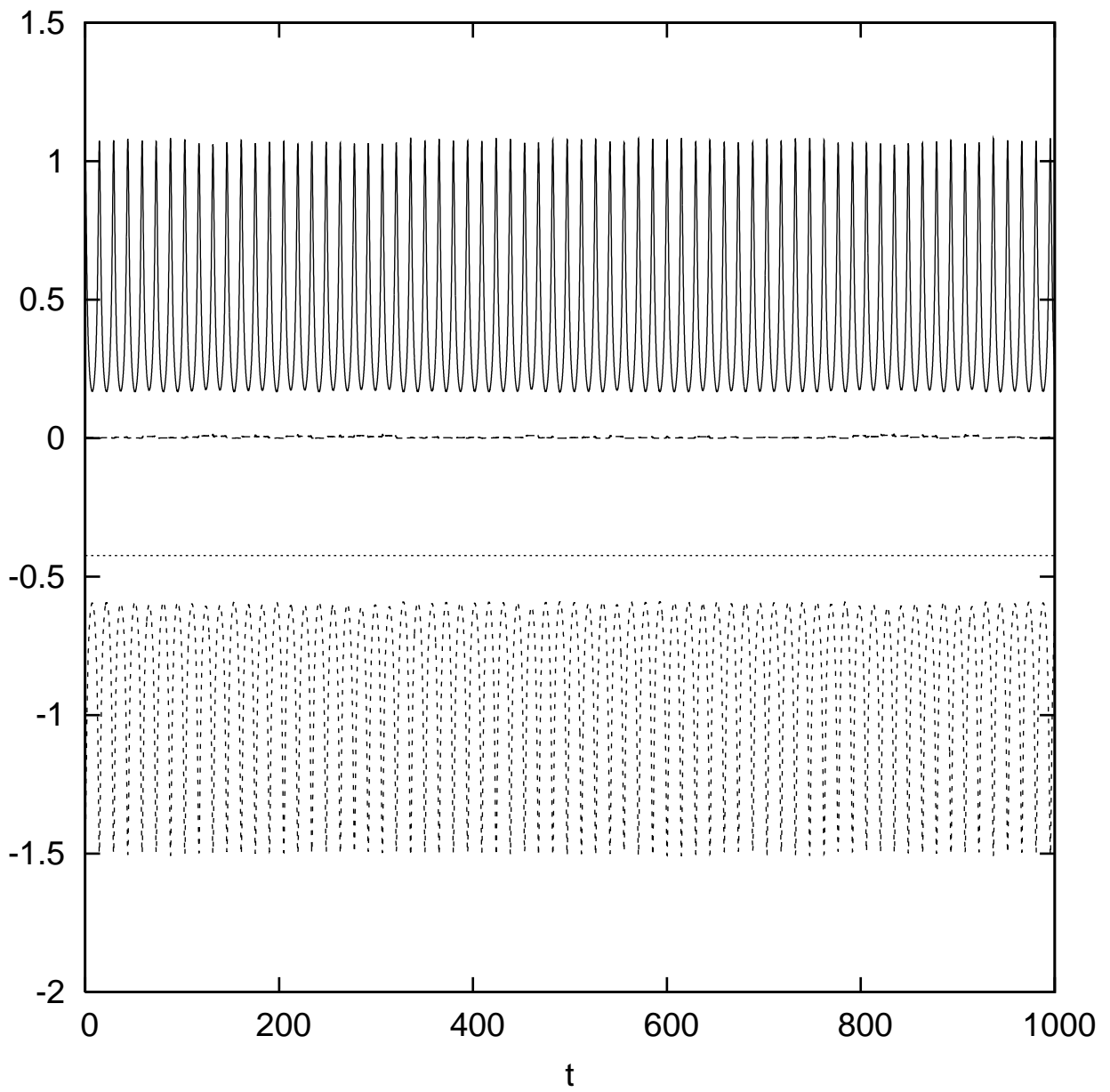
Orbiting Dumbbell Problem Elliptical Orbit -- Energy uanties -- Tolerance=10(-12) Top to Bottom: KE_t, KE_r, E_tot, PE_g
