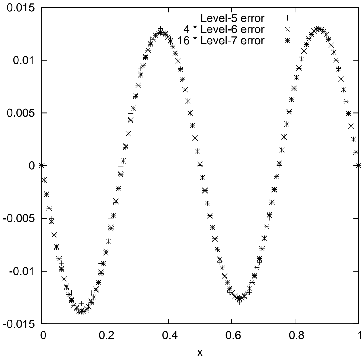
Convergence Test of Solution of Nonlinear BVP guess_factor = 1.0
